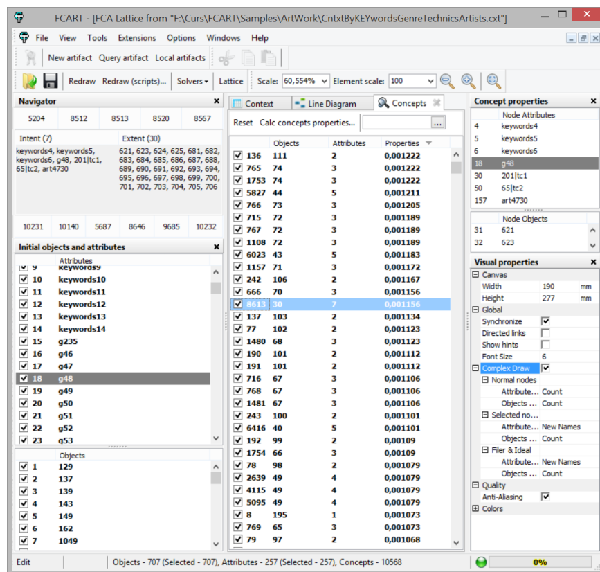
Fig. 3. List of all formal concepts, sorted by value of concept stability index
